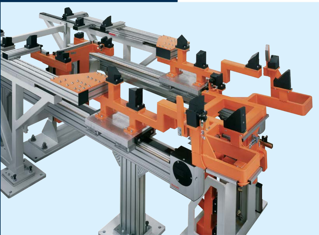
Combination of cam roller guides (front) and linear guides with recirculating ball bearings (back) for automotive interior door assembly
