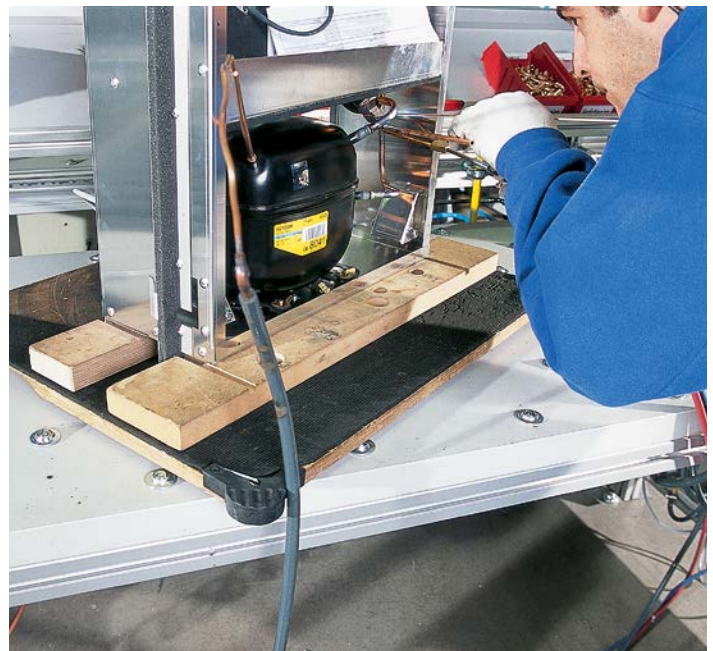
Manual assembly system for production of cooling units up to 75 kg weight and 2 m height
