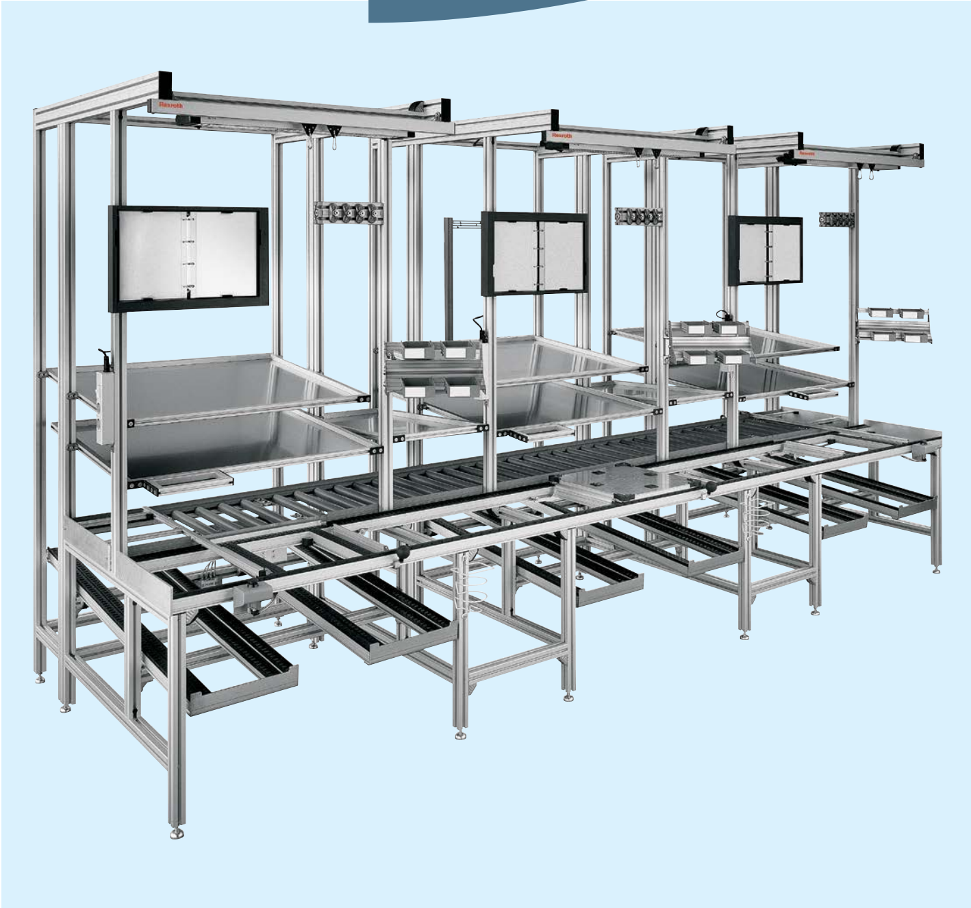
MPS workstation with manual process linking for burner assembly for water heaters
