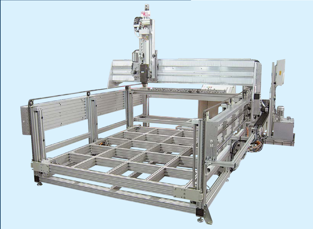
Linear guide for milling systems
