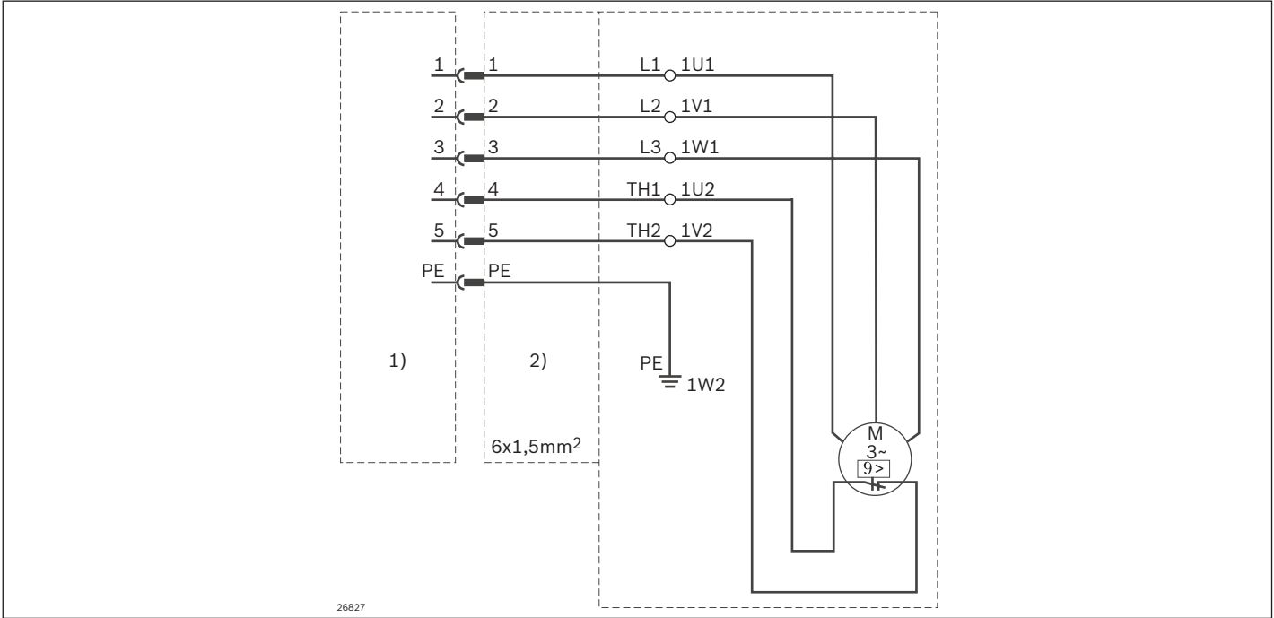
Motor connection with cable/plug (AT = 1), circuit diagram
