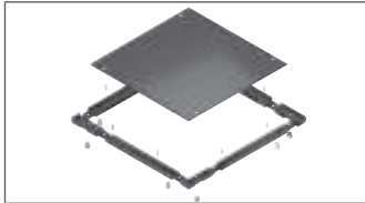
WT 2 polyamide workpiece pallet components
