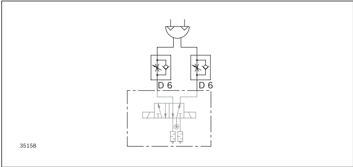
Pneumatic diagram of the HD 2/H lift rotate unit: Lifting cylinder for Size 1/2, rotation angle 90° (multiple position cylinder)
