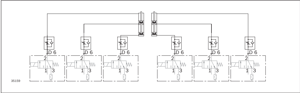
Pneumatic diagram of the HD 2/H lift rotate unit: Lifting cylinder for Size 1/2, rotation angle 180°
