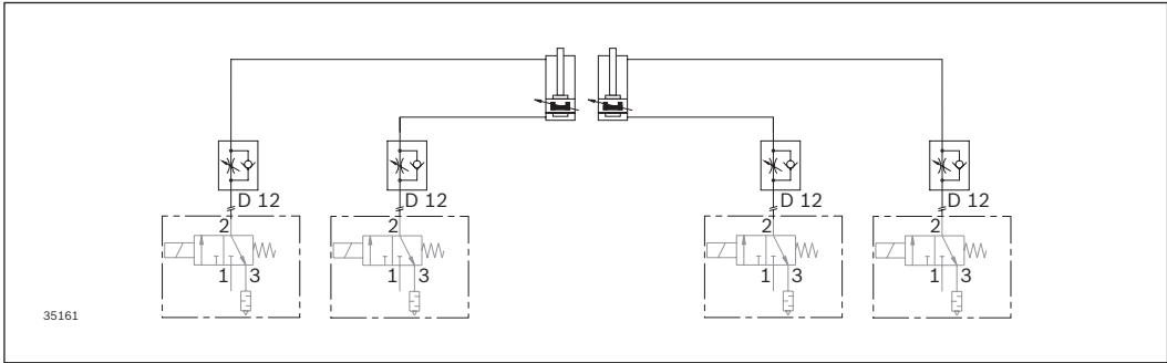
Pneumatic diagram of the HD 2/H lift rotate unit: Lifting cylinder for Size 3, rotation angle 90° and 180°
