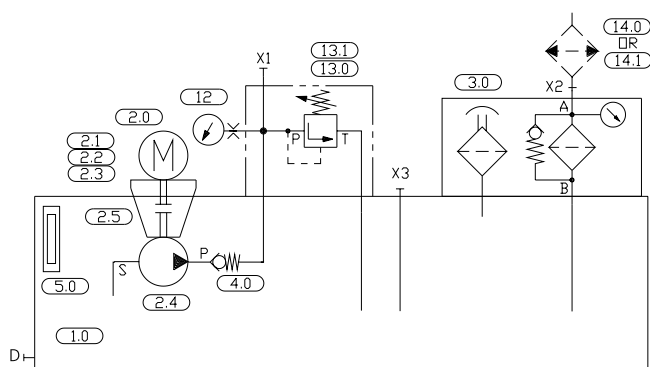
RV Circuit
