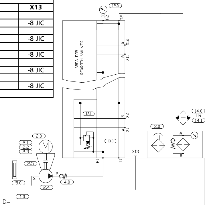
BM Circuit
