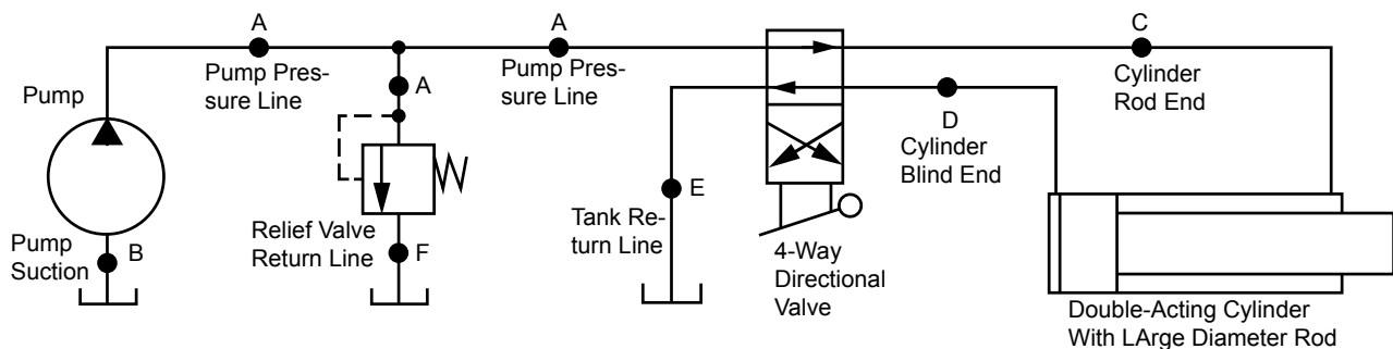
Figure 1. In different parts of the hydraulic circuit, flows and pressures are different. The optimum piping size for each line can be determined from permissible flow velocity and available pressure in each line.
