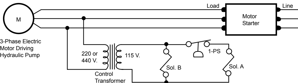
Figure 2. Electrical Circuit for Accumulator Bleed-Down and Pump Unloading
