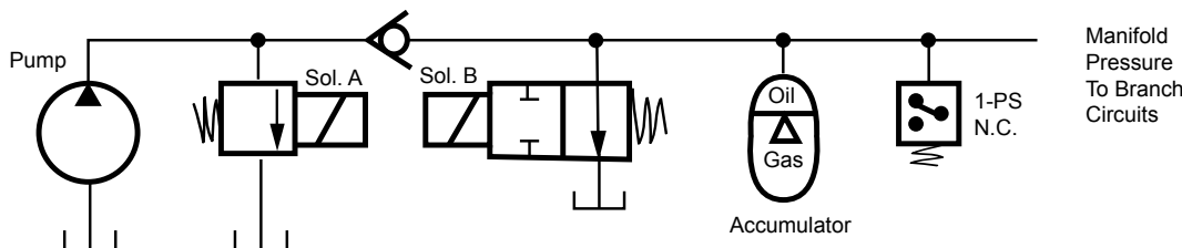
Figure 1. Typical Accumulator Hydraulic Circuit With Automatic Bleed-Down
