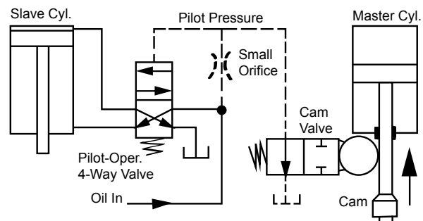
Figure 7. Master/slave cylinder system.
